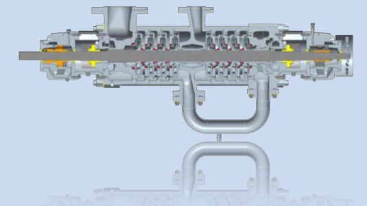
■ Type series GP „back-to-back“ version
